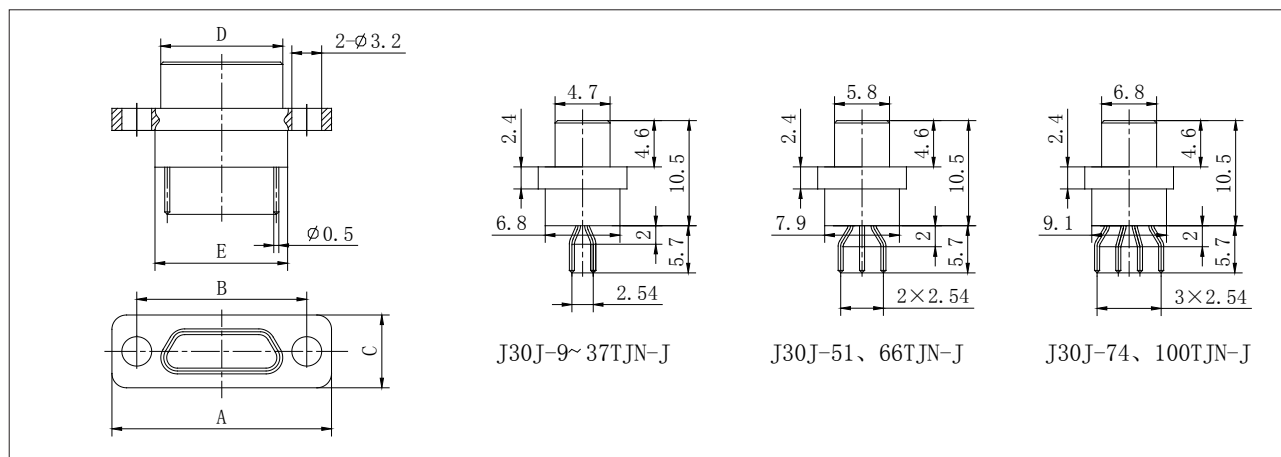
J30J-9~100TJN-J
