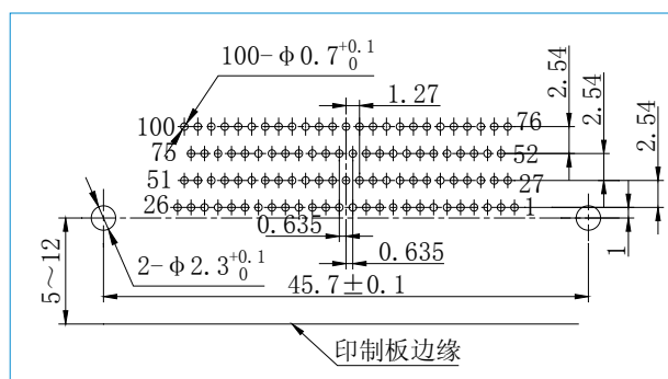
J30J-100TJW-J
