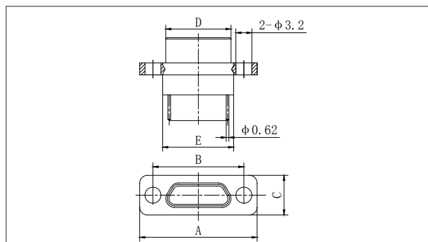
J30J-9~51TJN4/J30J-9~37TJN8
