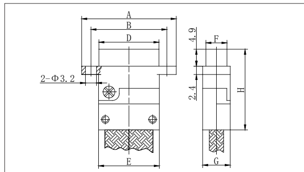
J30J-9~100ZK-GA
