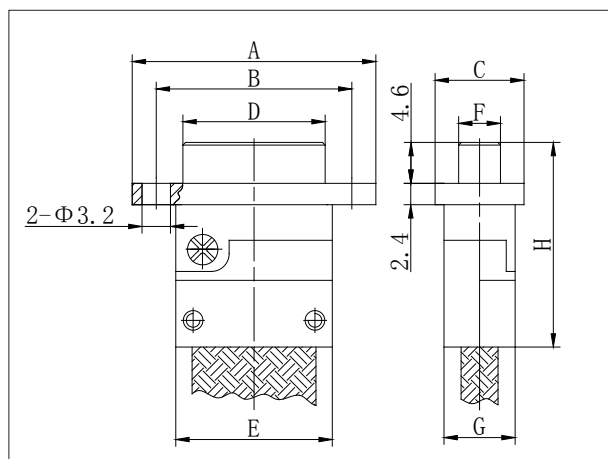
J30J-9~100TJ-AQ8
