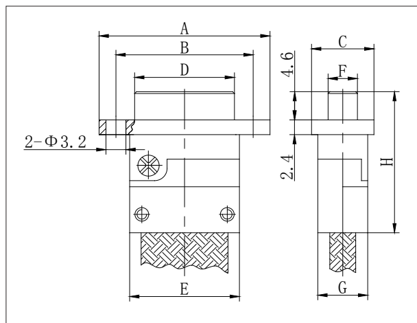
J30J-9~100TJ-GAQ
