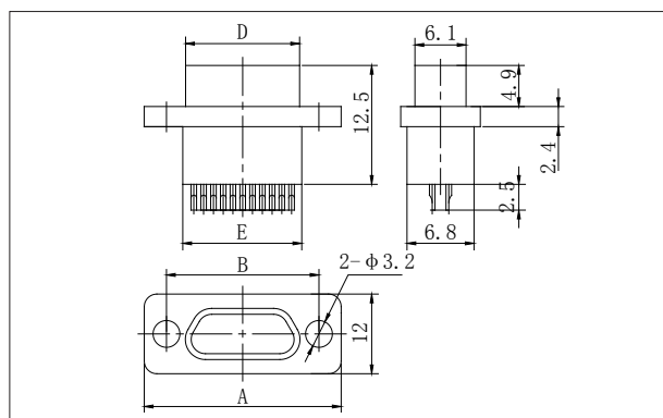
J30JM1-9 ~ 37ZKS
