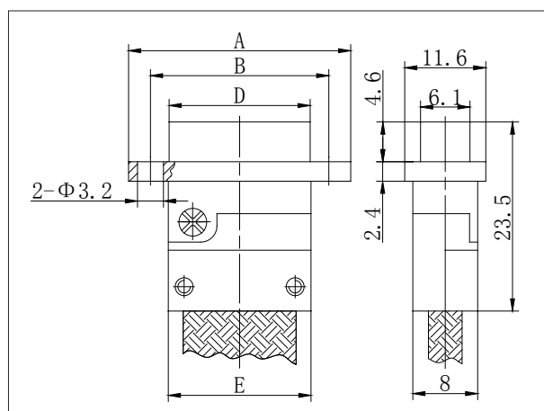
J30J-9~37ZK-GA (11.6)
