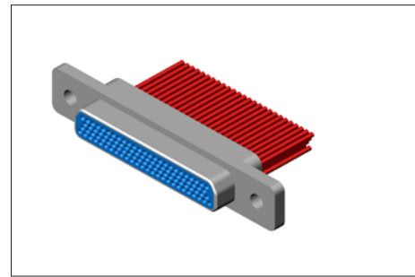
J30J-100TJ
