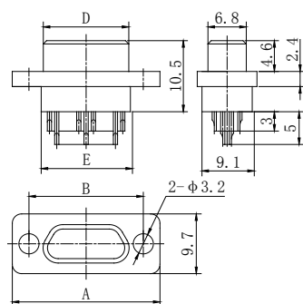
J30J-74, 100TJS
