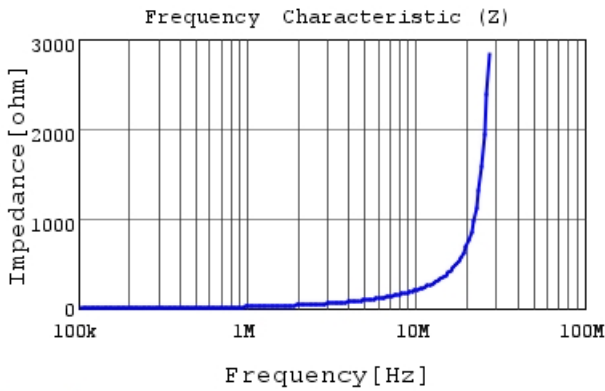
DFE322520FD-3R3M |Z|
