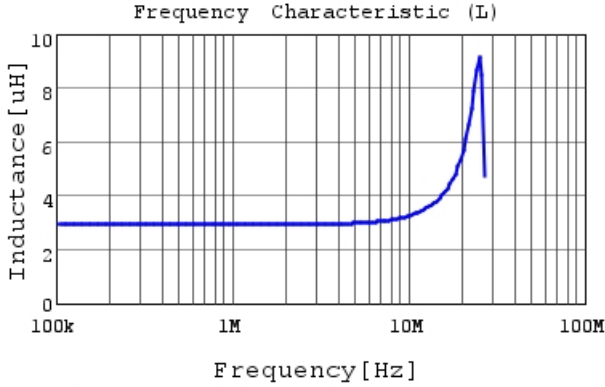
DFE322520FD-3R3M L
